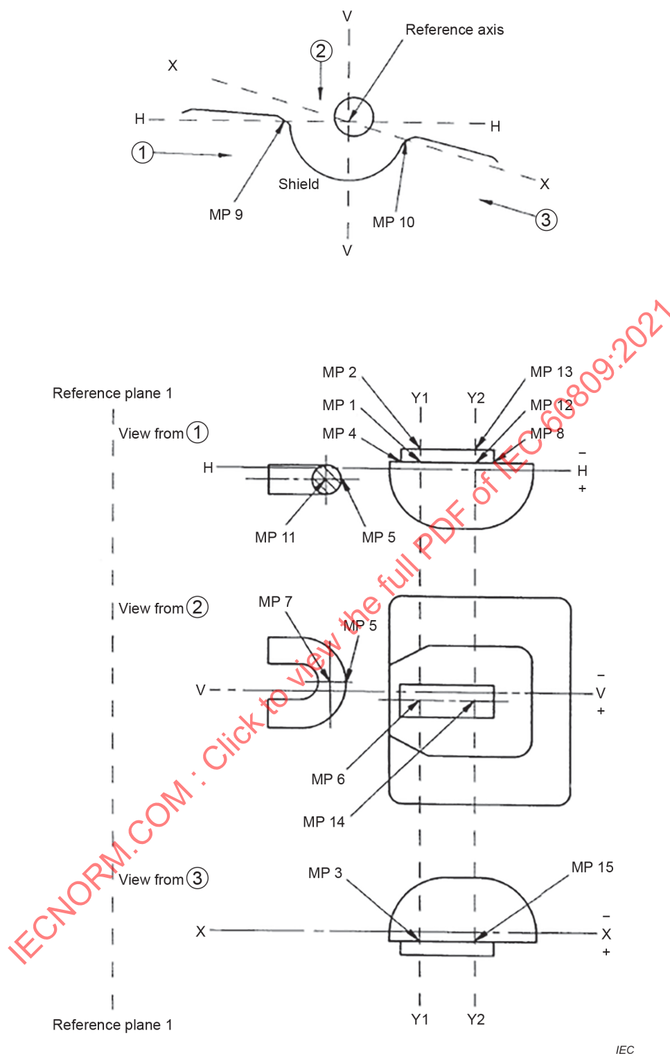
Figure D.2 – Position of measuring points of R2 lamps
