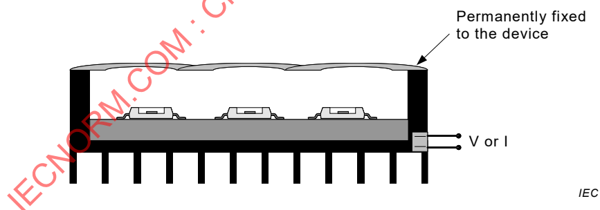
Figure 5 – Example of a non-replaceable LED light source
