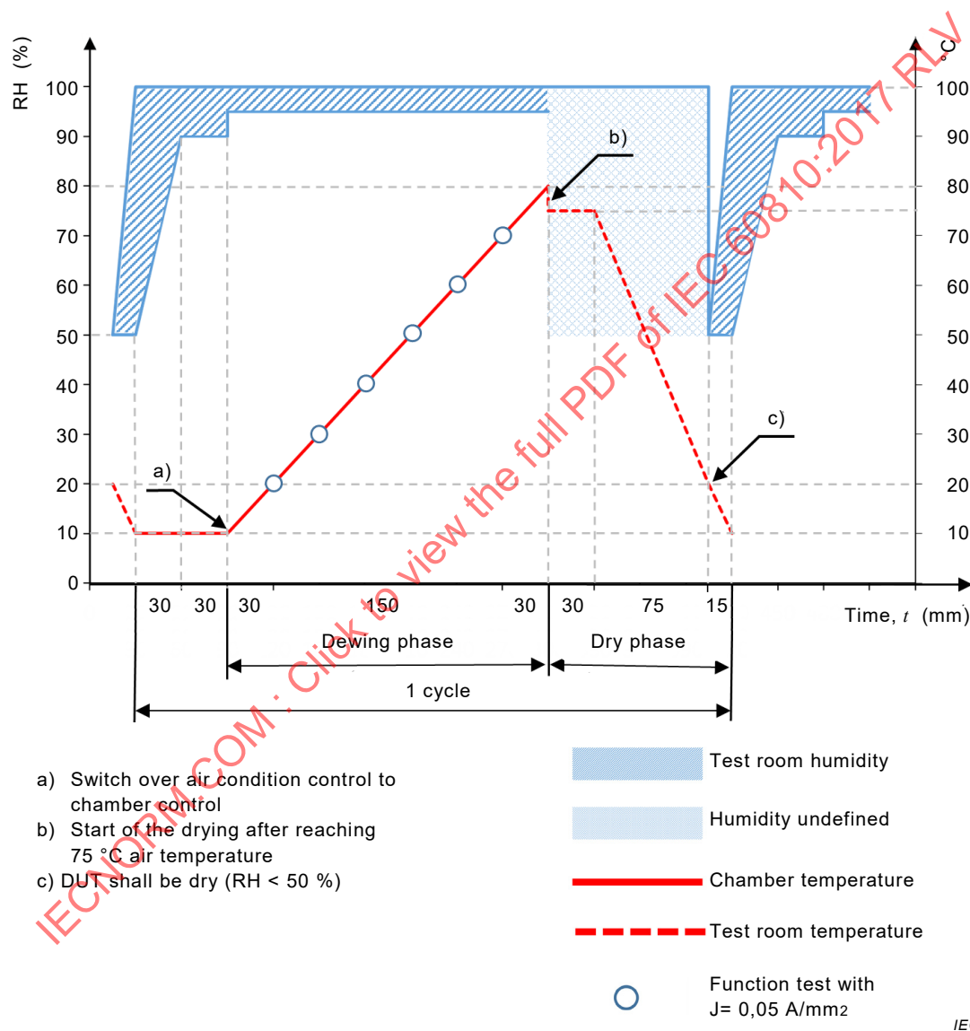
Figure 12 – Temperature–humidity characteristics for the DEW test
