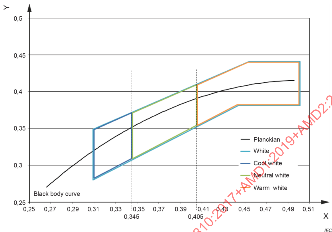
Figure 13 – Three white colour groups for LED light sources
