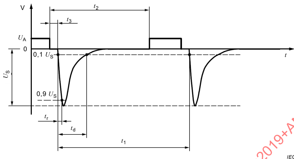
Figure 10 – Profile of pulse 1 from ISO 7637-2
