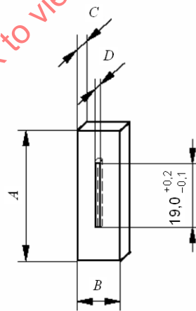
Figure 7 – Notched test pieces
