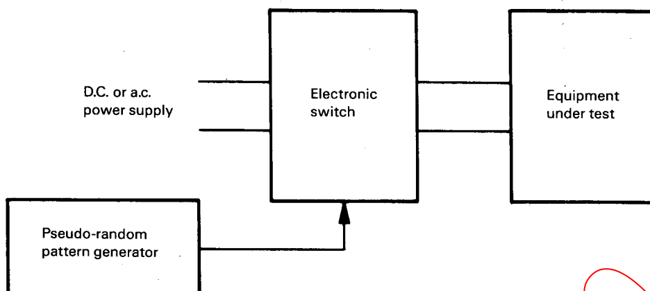
FIG. 10. — Test circuit for testing power supply interruptions.
