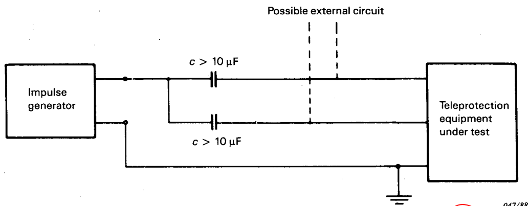
FIG. 7. — Circuit configuration for common mode impulse withstand test with blocking of d.c. circulation on impulse generator.
