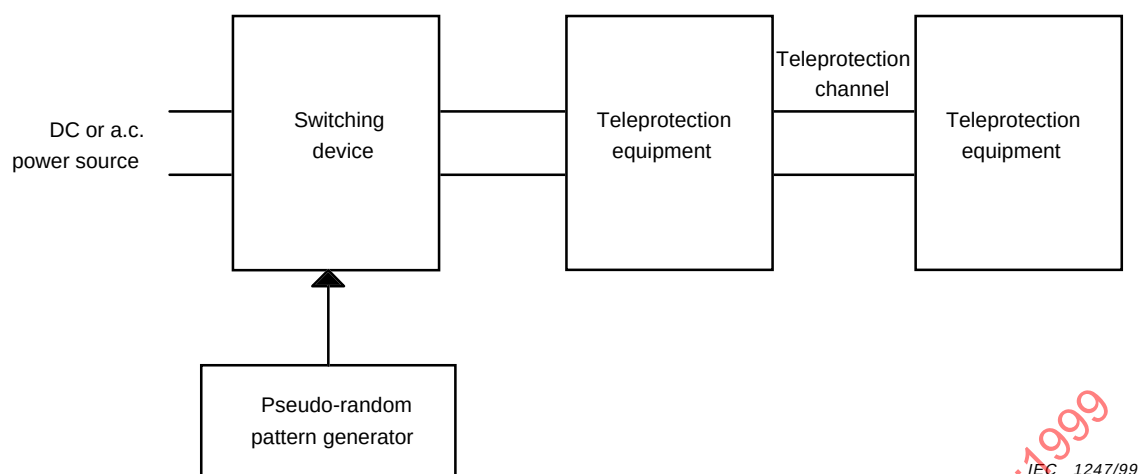
Figure 7 – Test circuit for testing power supply interruptions
