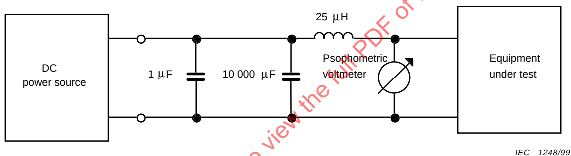
Figure 8 – Test circuit for LF disturbance emission measurement
