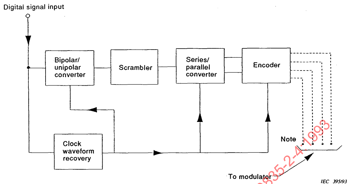
Figure 1a – Transmit processor
