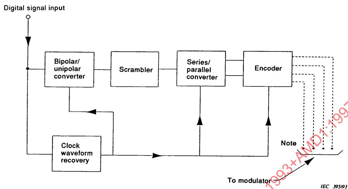
Figure 1a – Transmit processor
