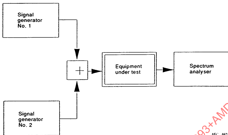
Figure 2 – Arrangement for measuring the selectivity of the carrier part of a digital receiver
