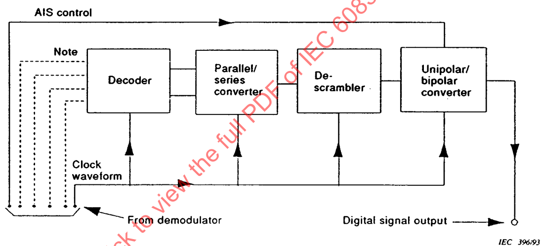
Figure 1b – Receive processor
