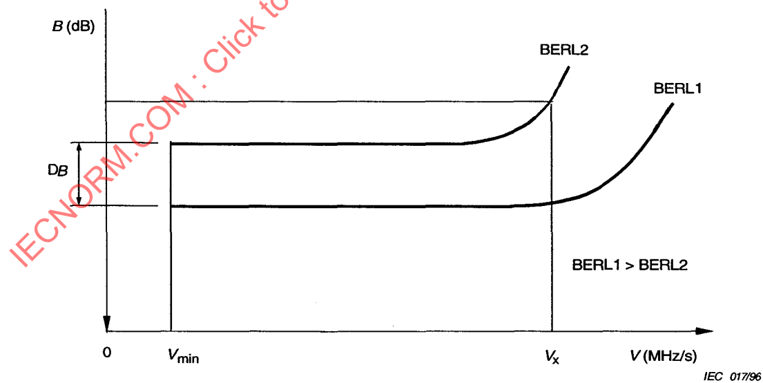
Figure 11b – Graphical representation of the relative system sensitivity to dynamic fading: sweep of the notch offset frequency
