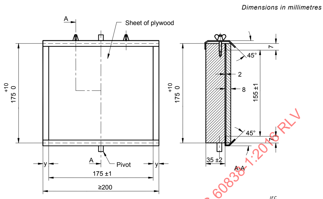
Figure D.2 – Mounting fixture
