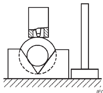
b) Test piece in V-blocks
