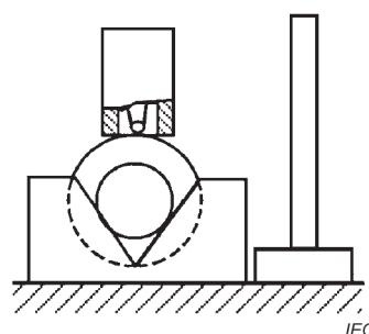
b) Test piece in V-blocks
