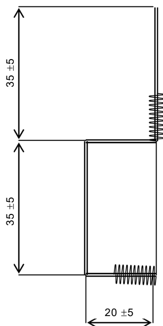
Figure 4 – Example of carrier for solderability test
