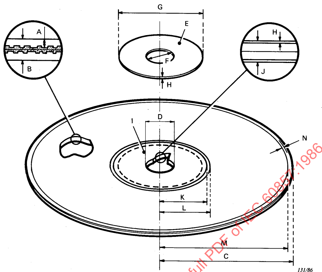
FIG. 1. — Mechanical parameters of the disk (Sub-clauses 4.1 to 4.13).
