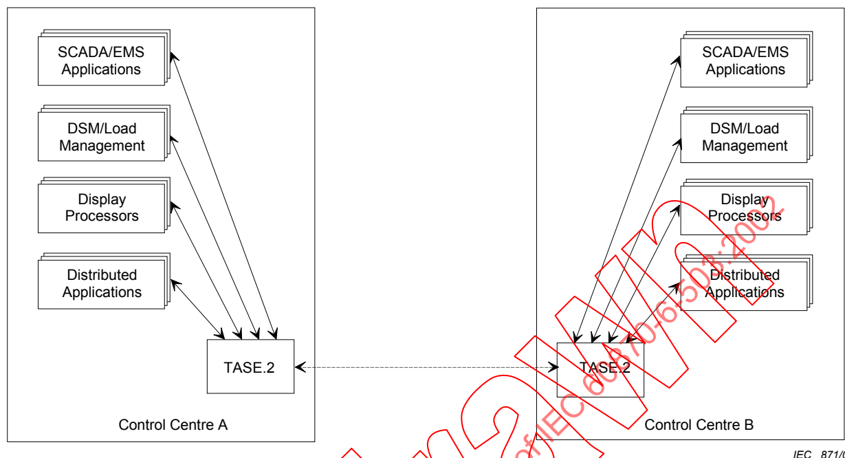
Figure 4 – Informal TASE.2 Model
