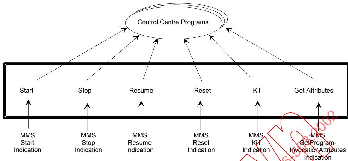
Figure 18 – Server Program Components
