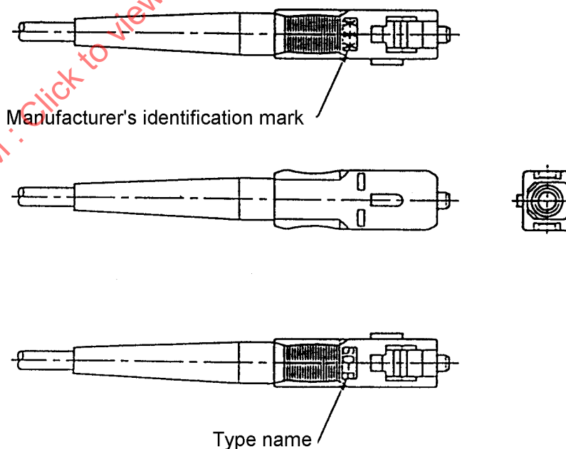
Figure 4 – Example of component marking
