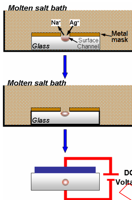
Figure A.3 – PLC by ion-exchange
