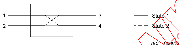
Figure 9 – Four-port switch with crossover
