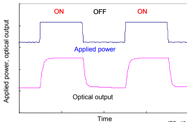
Figure A.7 – Example of switching response of TO switch
