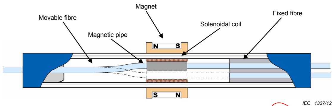
Figure A.3 – Example of mechanical switch (fibre driving type)
