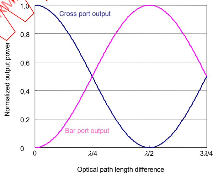
Figure A.6 – Output power of TO switch
