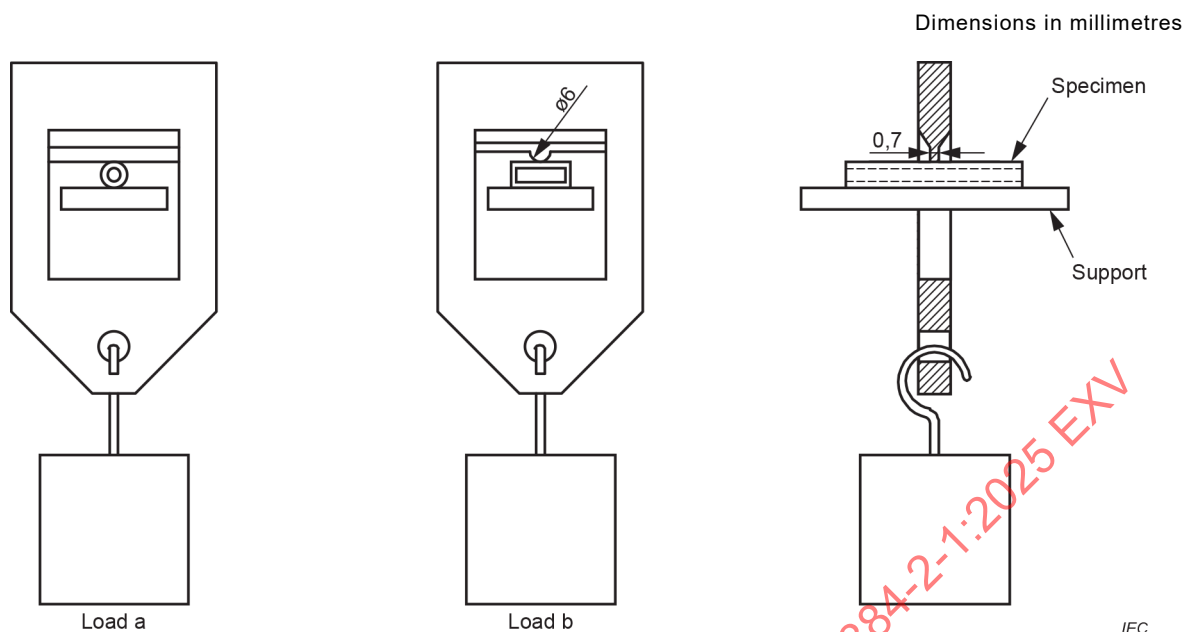
Figure 44 – Apparatus for pressure test at high temperature
