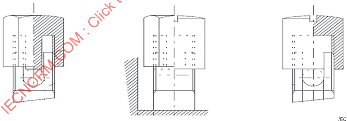
Figure 12 – Mantle terminals
