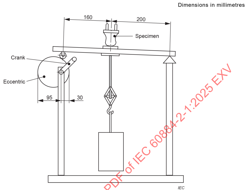
Figure 27 – Apparatus for testing cord retention
