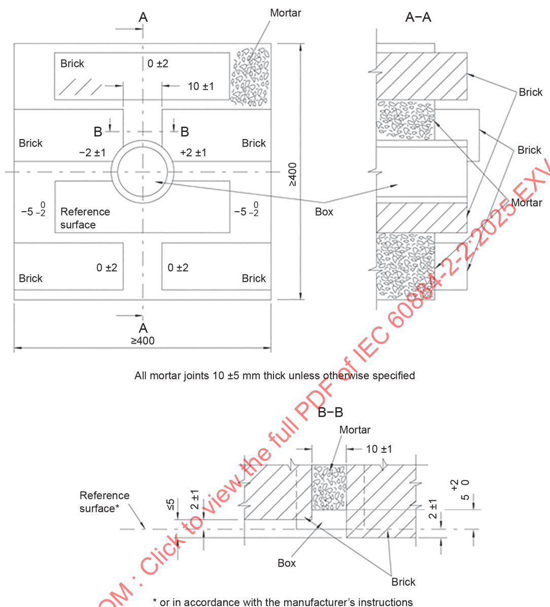
Figure 18 – Types of test wall
