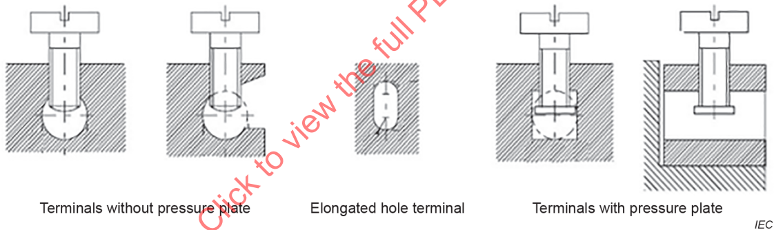
Figure 9 – Pillar terminals
