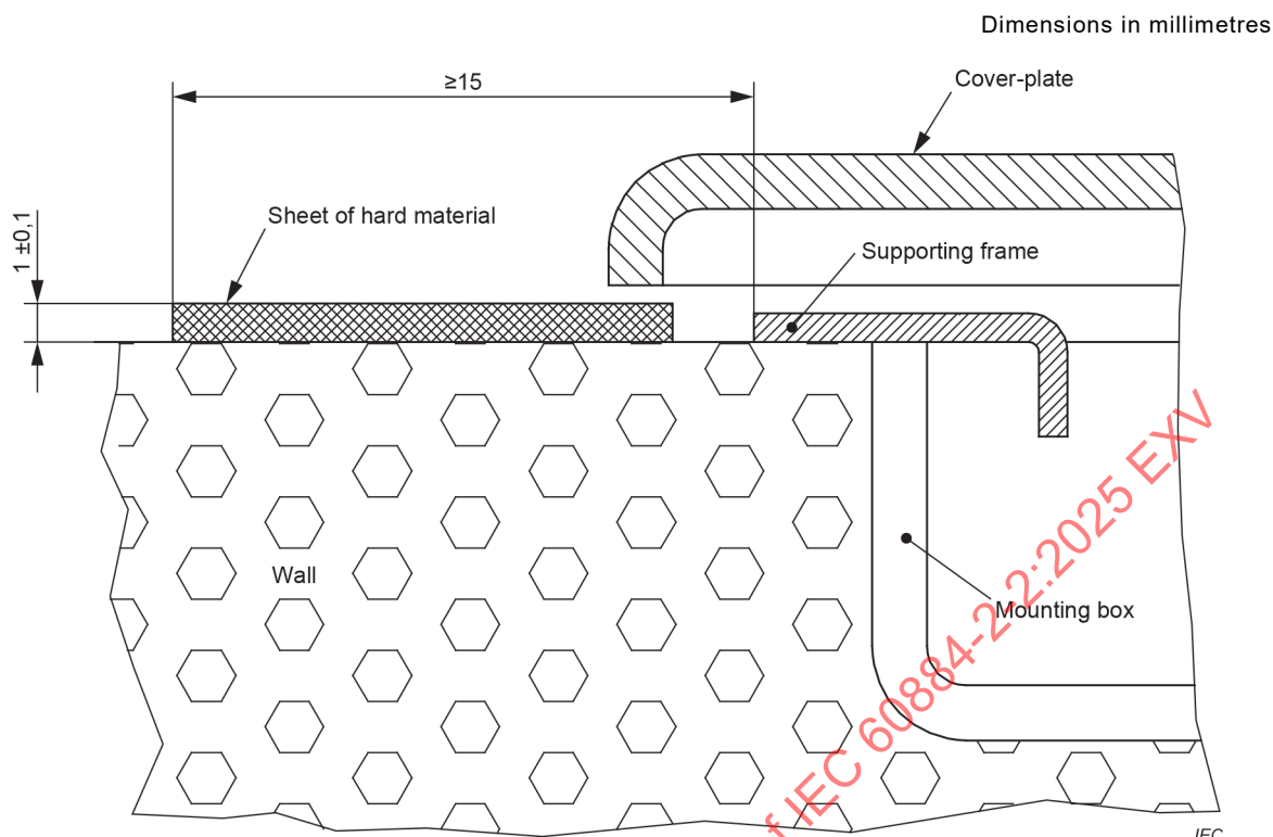
Figure 34 – Arrangement for test on covers or cover-plates
