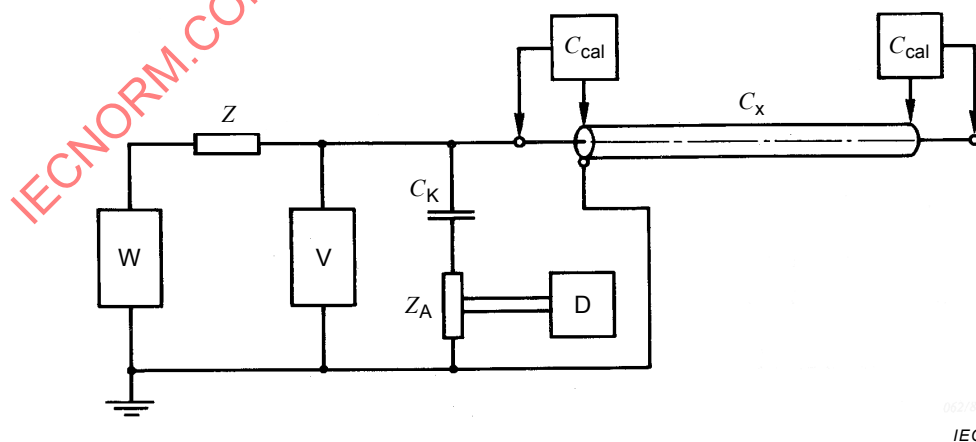
Figure 5 – Input unit Z_A connected in series with the coupling capacitor, C_K
