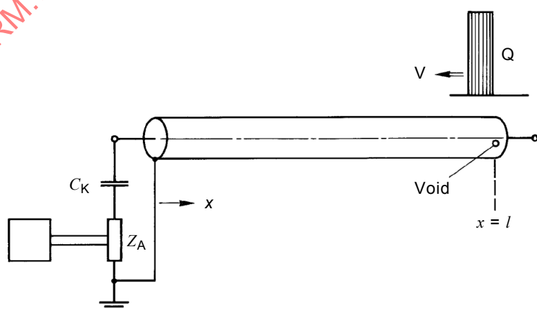
Figure 1 – Discharge site exactly at the cable end remote from the detector ( x = l )
