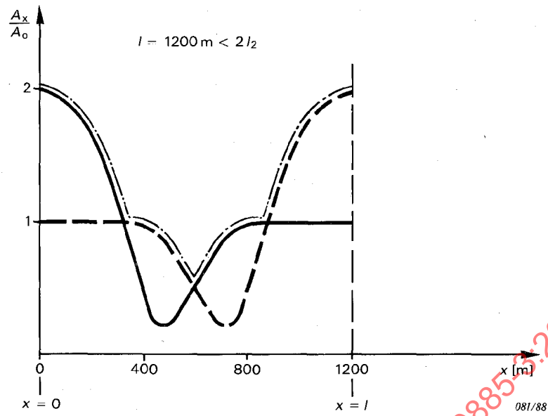
Figure 19 — Negative superposition for 2l_1 < l < 2l_2
