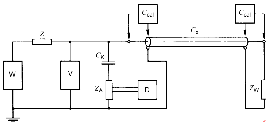
Figure 8 – Connection of the terminal impedance Z_W
