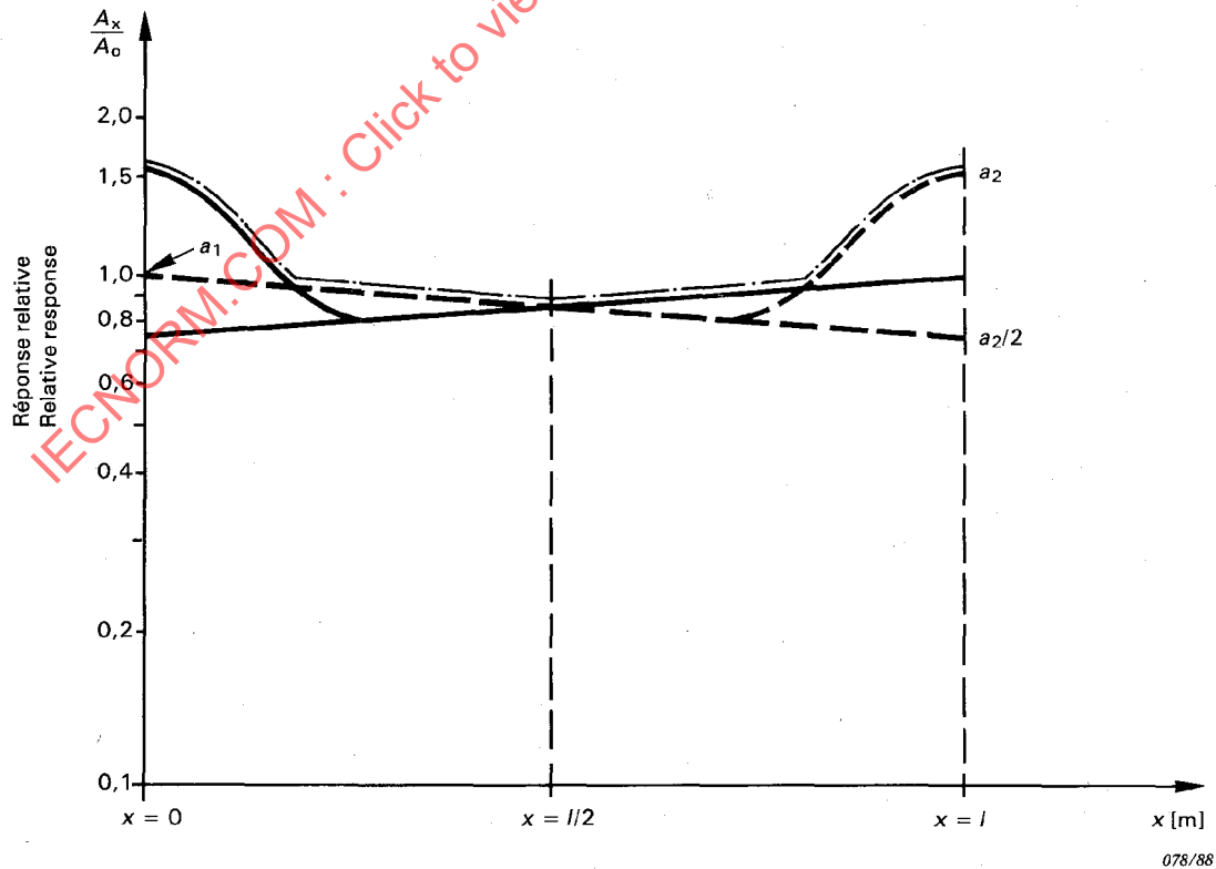
Figure 16 — Maximum attenuation error at the centre of the cable if measurements are made from both ends
