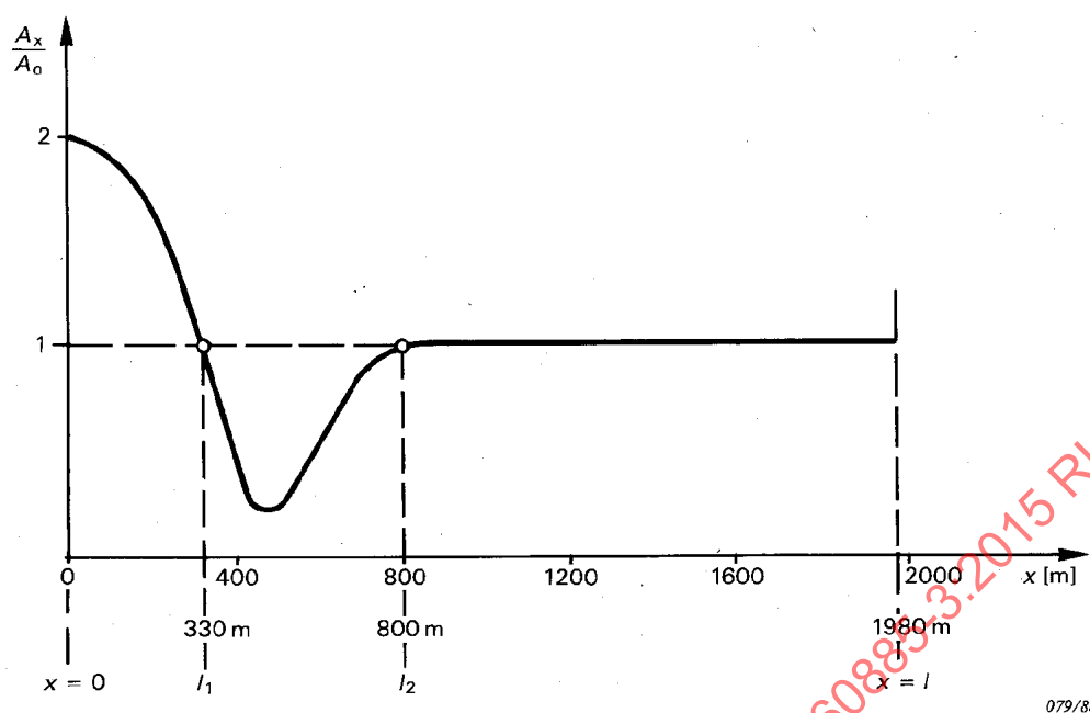
Figure 17 — Double pulse diagram type 2. Negative superposition between l_1 and l_2 (forbidden length).
