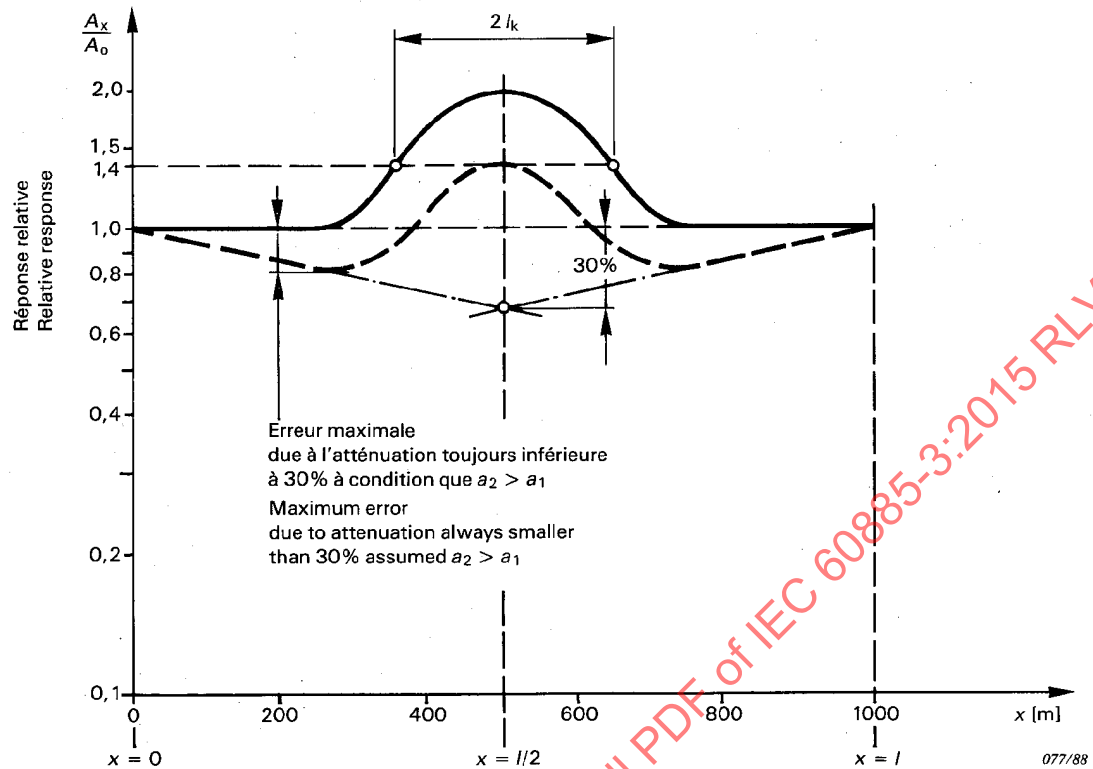
Figure 15 — Maximum attenuation error, both cable ends connected together
