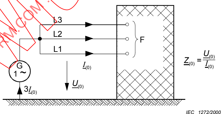
Figure 5c – Zero-sequence short-circuit impedance Z_{(0)}
