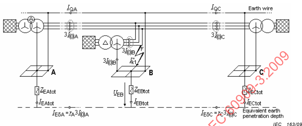
Figure 4 – Partial short-circuit currents in case of a line-to-earth short circuit inside station B
