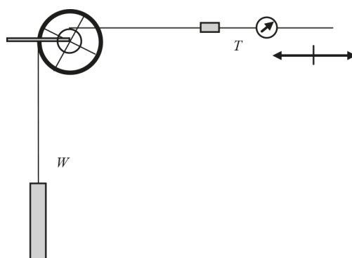
Figure 10 – Example of a tensioning device measurement test
