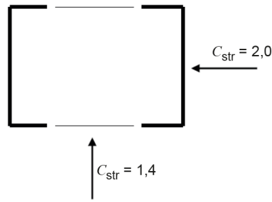
Figure 6 – Definition of drag factors for double channel pole
