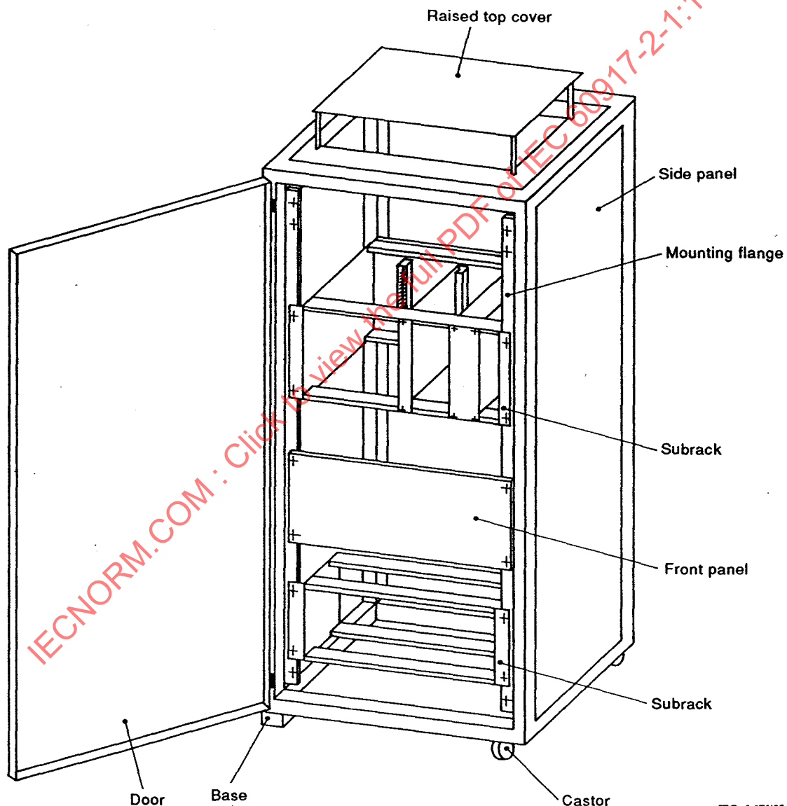
Figure 1 – Example of a cabinet with subracks, front panels and attachments installed
