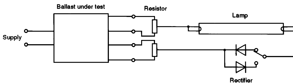
Figure 1 – Circuit for testing rectifying effect
