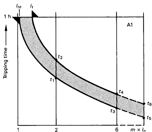
Figure A.1 – Thermal mode only
