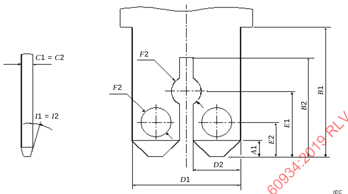
Figure E.13 – Dimensions of male tabs for two different sizes of female connectors (see 8.1.7.1)
