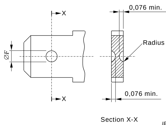
Figure E.7 – Dimensions of round dimple detents of male tabs (see Figure E.6)
