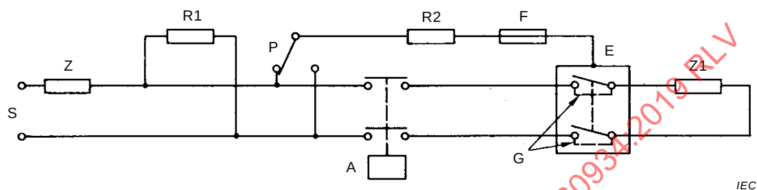
Figure 3b – Two-pole CBE
