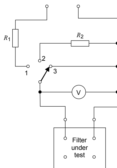
Figure 3 – Test circuit for d.c. test
