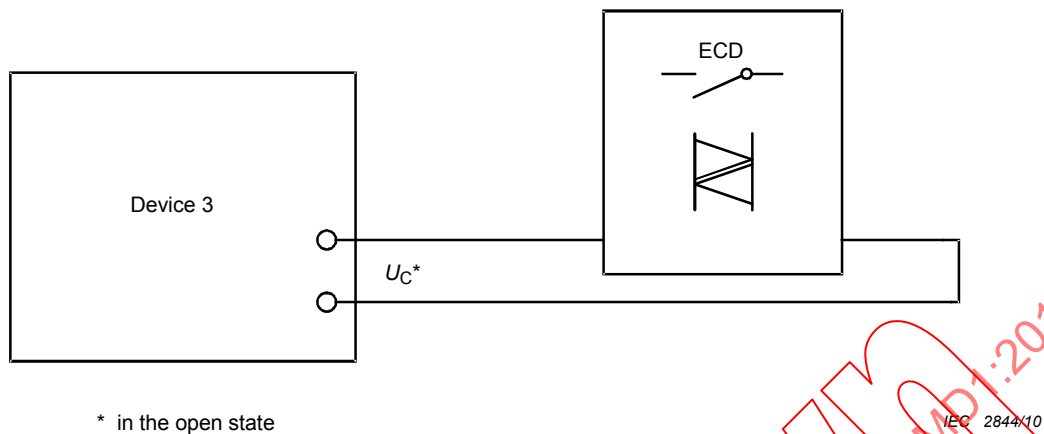
Figure U.4 – Equipment with an internal control supply and control input only
