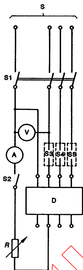
Figure B.3 – Test circuit for the verification of the behaviour of CBRs classified under B.3.1.2.2.1 (see B.8.9)
