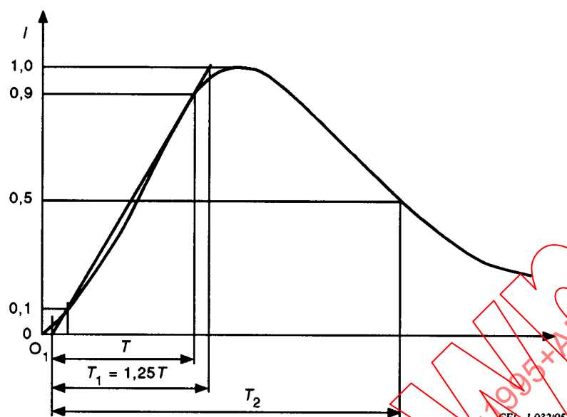
Figure B.6 – Surge current wave 8/20 \mu s
