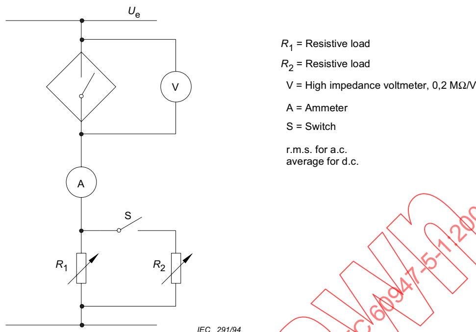
Figure H.2 – Example of test circuit for the verification of voltage drop, minimum operational current and OFF-state current (see H.8.2, H.8.3 and H.8.4)
