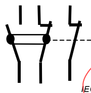
Figure L.1 – Example of representation of NO and NC contacts which are mechanically linked and NC non-linked contact
