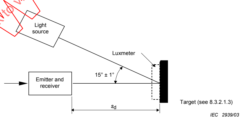
Figure 11d – Type D, emitter-receiver and target
