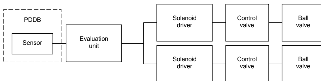
Figure A.2 – Architecture of the safety related function
