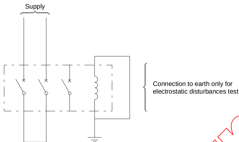
Figure 2 – Test circuit for the verification of the influence of low-frequency, electrostatic and of electromagnetic field disturbances
