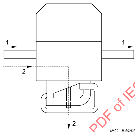
Figure 5 – Arrangement for the thermal short-time withstand current test
