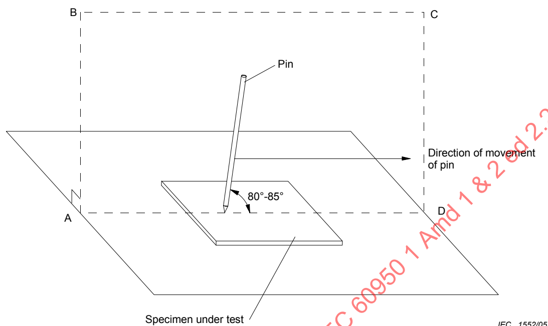
Figure 2K – Abrasion resistance test for coating layers
