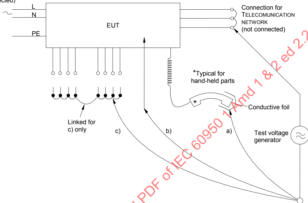
Figure 6B – Application points of test voltage
