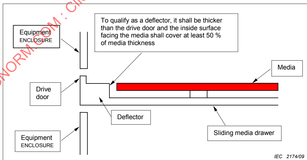
Figure 4H – Example for determining opening 'X' with a deflector
