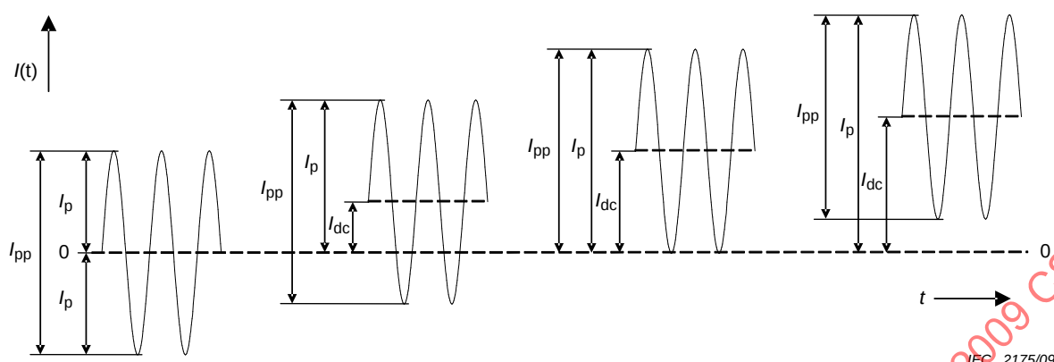
Figure M.3 – Peak and peak-to-peak currents
