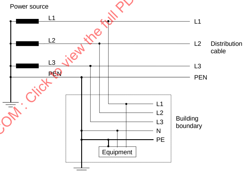
Figure V.2 – Example of TN-C-S power distribution system
