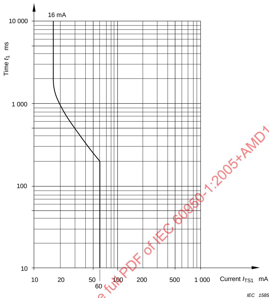
Figure M.2 – I_{TS1} limit curve for cadenced ringing signal
