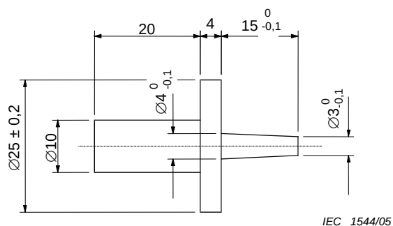
Figure 2A – Test finger
