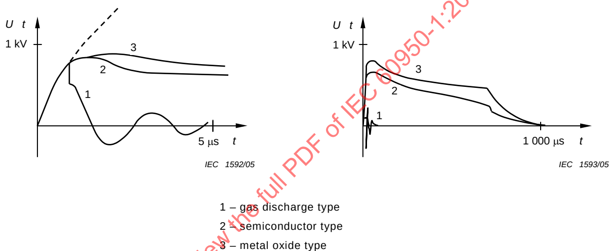
Figure S.2 – Waveforms on insulation during breakdown without surge suppressors
