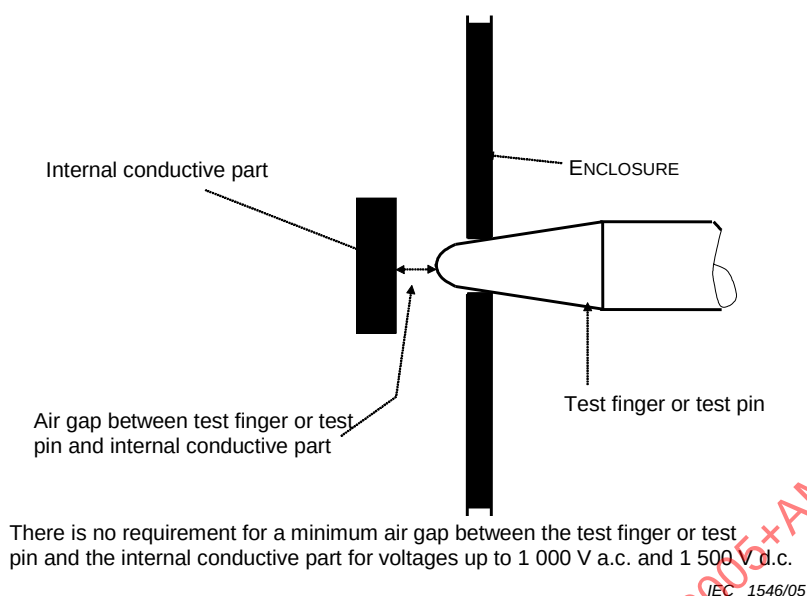
Figure 2D - Accessibility of internal conductive parts
