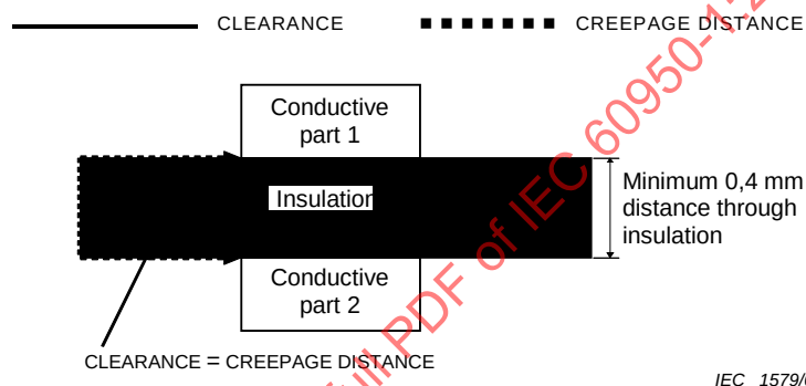
Figure F.14 – Solid insulating material
