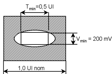
Figure 5 – Eye diagram
