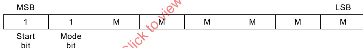
Figure L.2 – Extended mode
