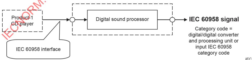
Figure R.6 – Digital/digital converter
