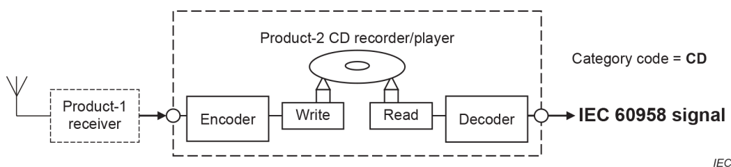
Figure R.4 – Monitoring after recording
