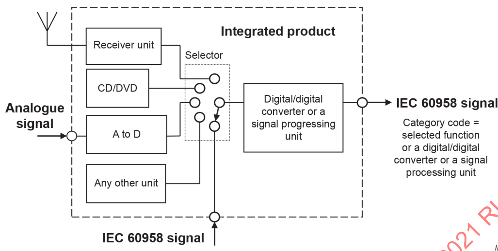
Figure R.7 – Integrated product including digital/digital converter
