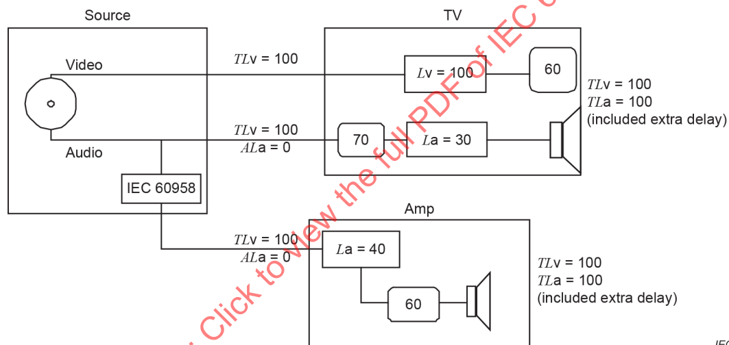
Figure S.7 – Another example for solving lip-sync problems
