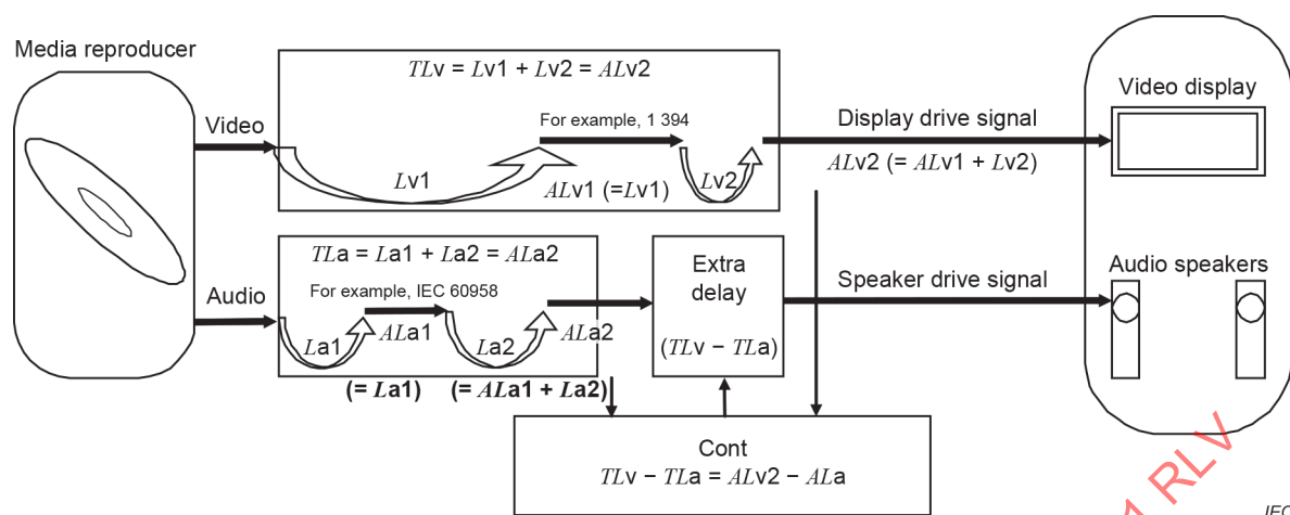
Figure S.4 – Latency parameter transmission
