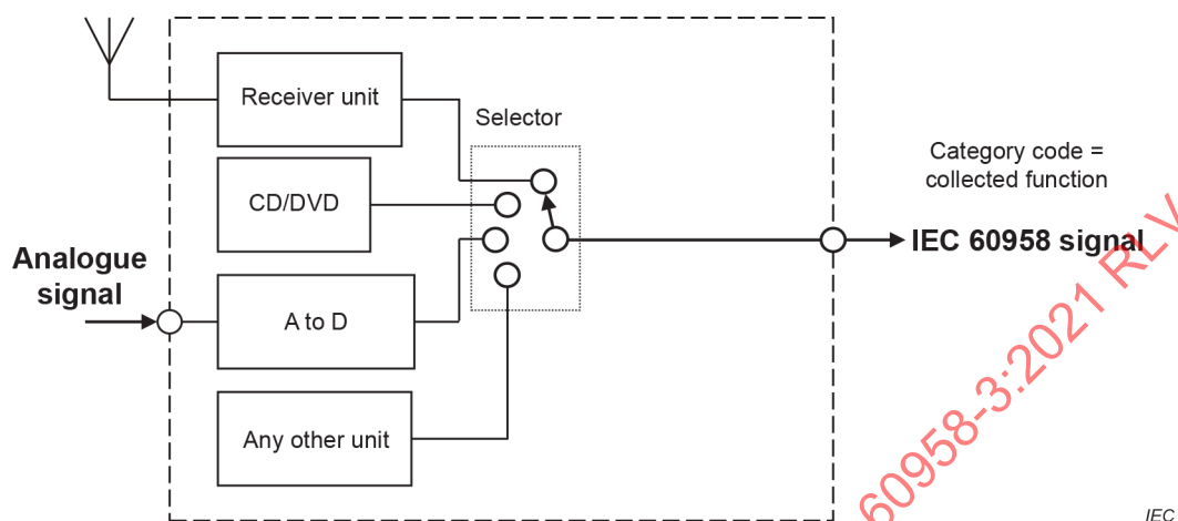
Figure R.5 – Integrated product
