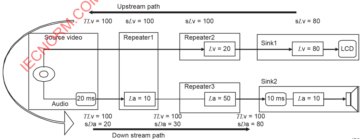
Figure S.6 – Example of latency parameter transmission
