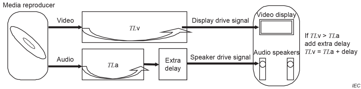
Figure S.2 – Lip-sync compensation
