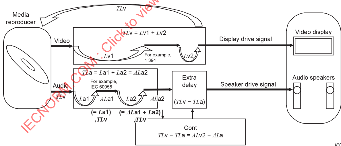
Figure S.5 – Latency parameter transmission with TLv
