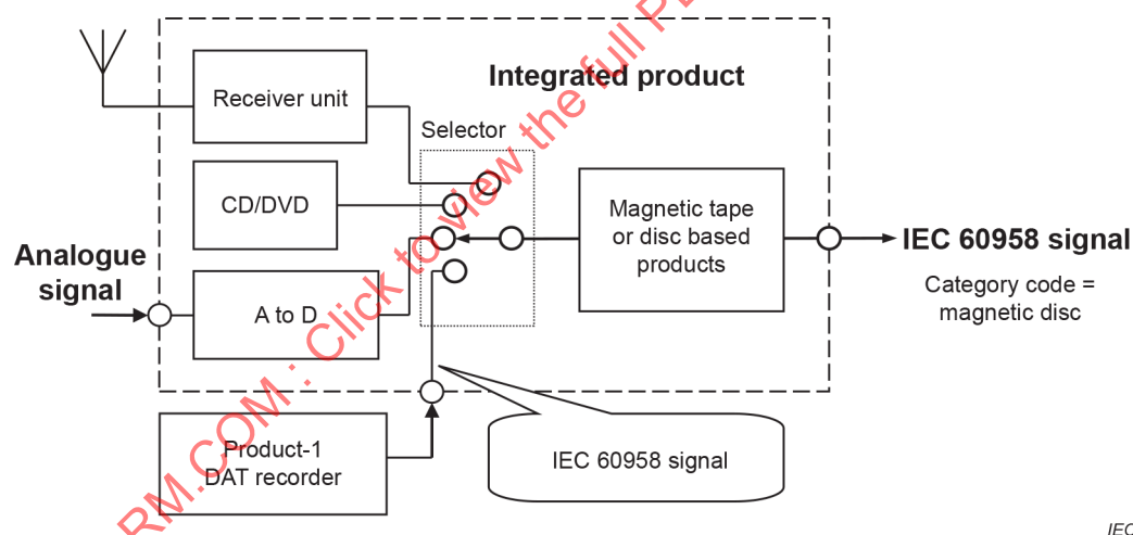
Figure R.8 – Integrated product including magnetic disc recorder
