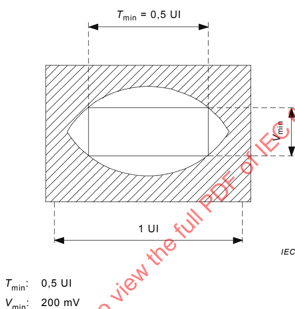
Figure B.2 – Eye diagram, balanced receiver
