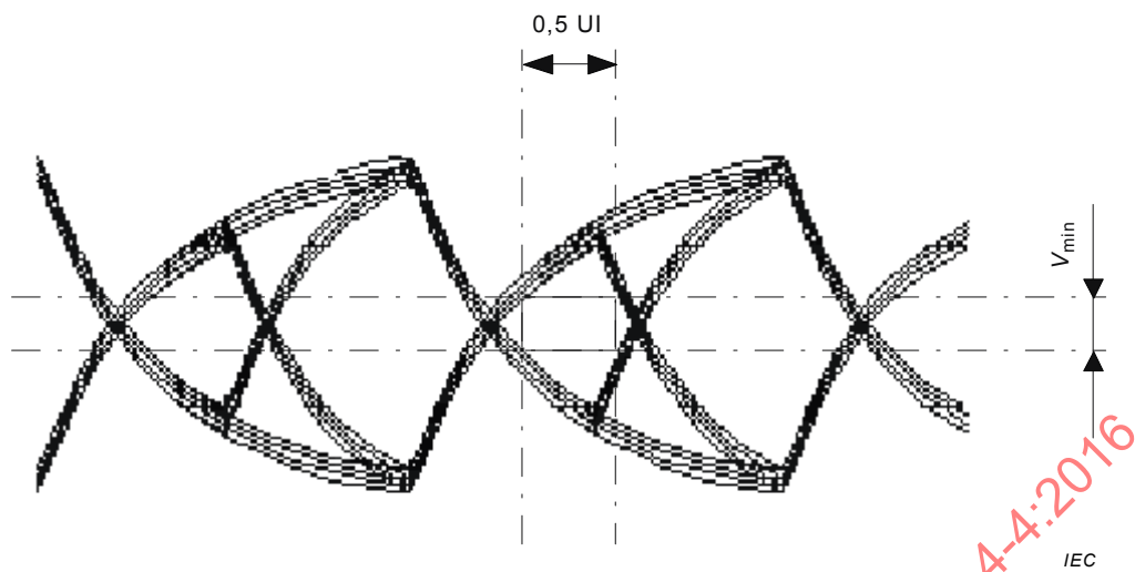
Figure C.3 – Eye pattern for long-distance transmission
