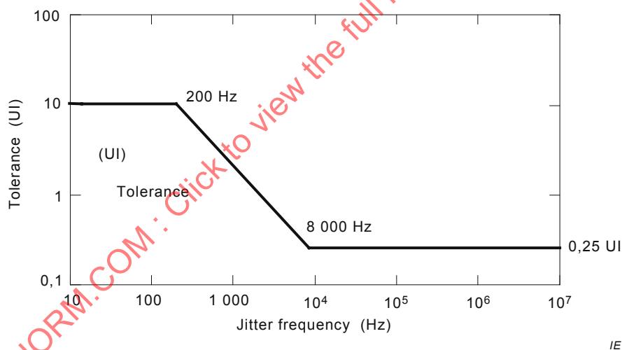
Figure 3 – Jitter tolerance template
