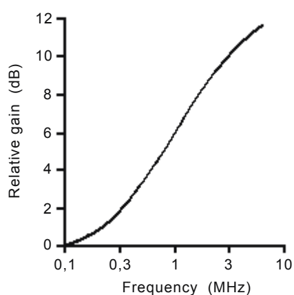
Figure B.3 – Suggested equalizing characteristic for a receiver operating at 48 kHz frame rate
