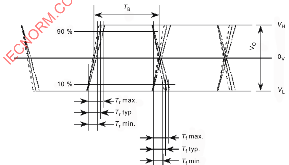
Figure C.1 – Output signal waveform
