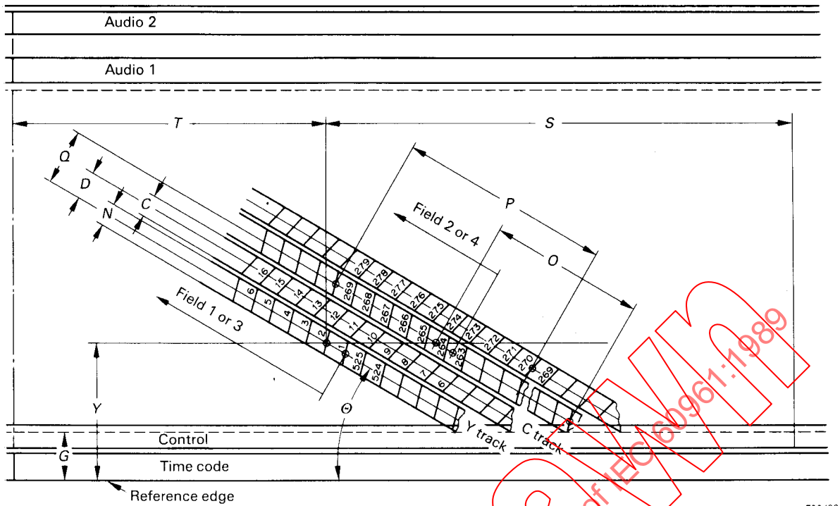
FIG. 4a. - Video record location (525/60).
