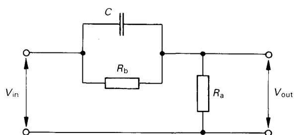
FIG. 6. — Pre-emphasis network.
