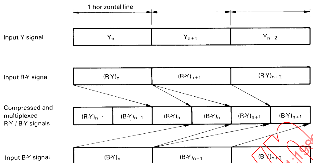
FIG. 8. – System of time compression and multiplexing.
