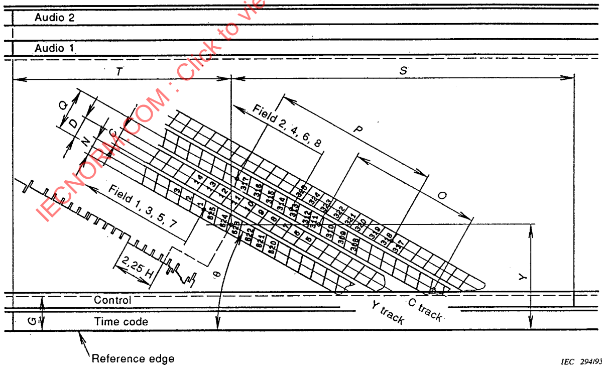
Figure 4b – Video record location (625 line-50 field)
