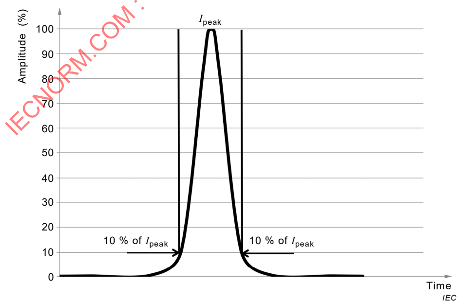
Figure H.1 – Typical inrush current profile
