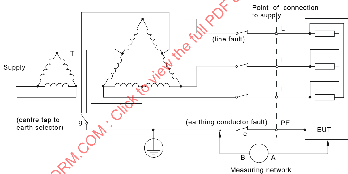
d) Three-phase equipment on earthed centred three-phase three-line system
