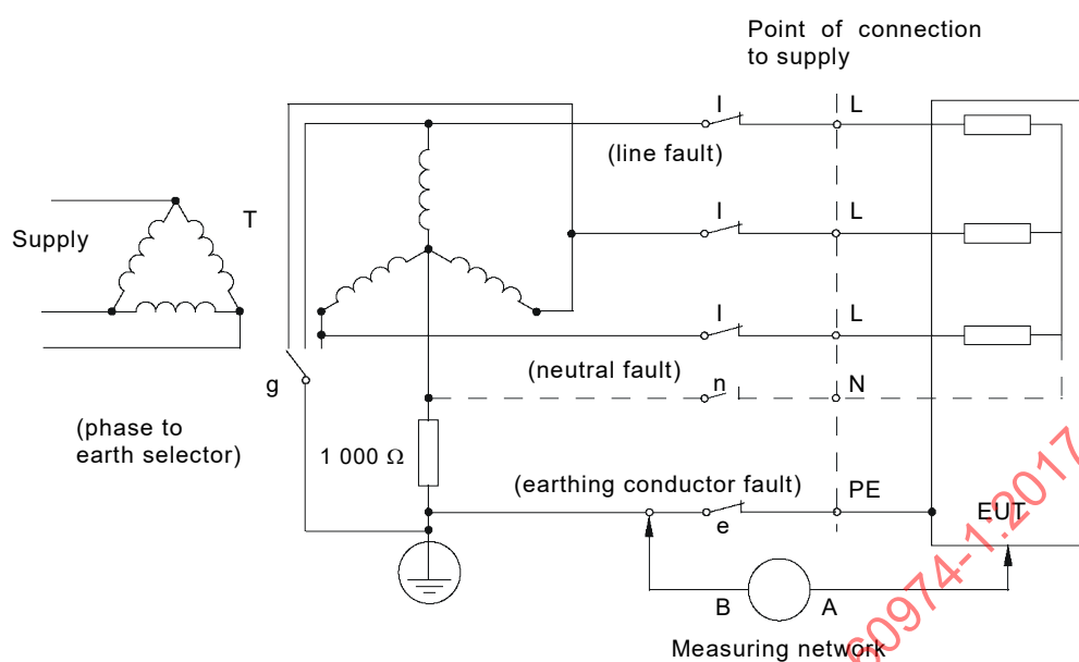
c) Three-phase equipment on star IT system
