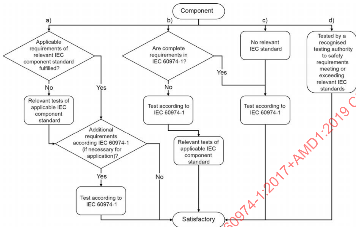
Figure P.1 – Flow chart for conformity methods of Annex P
