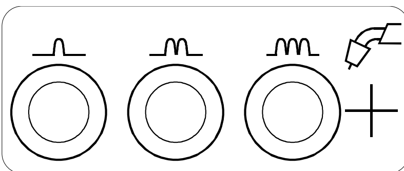
Figure L.4 – Terminals with inductance selector for MIG/MAG welding
