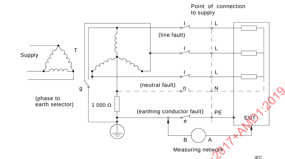
c) Three-phase equipment on star IT system
