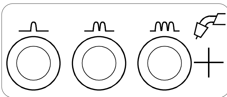
Figure L.4 – Terminals with inductance selector for MIG/MAG welding
