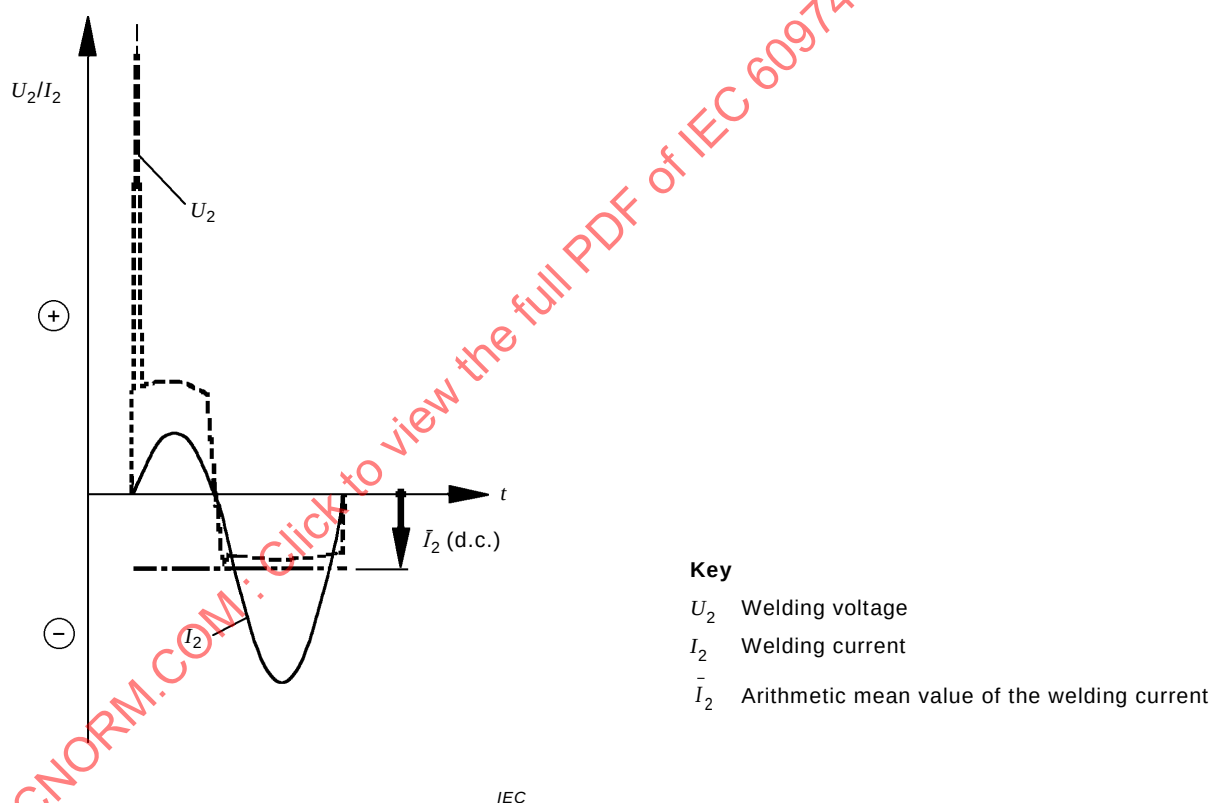
Figure C.1 – Voltage and current during AC tungsten inert-gas welding
