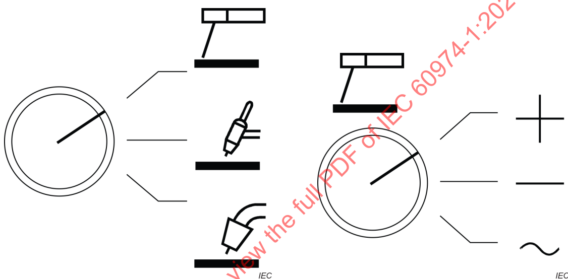
Figure L.5 – Process switch (MMA, TIG, MIG)
