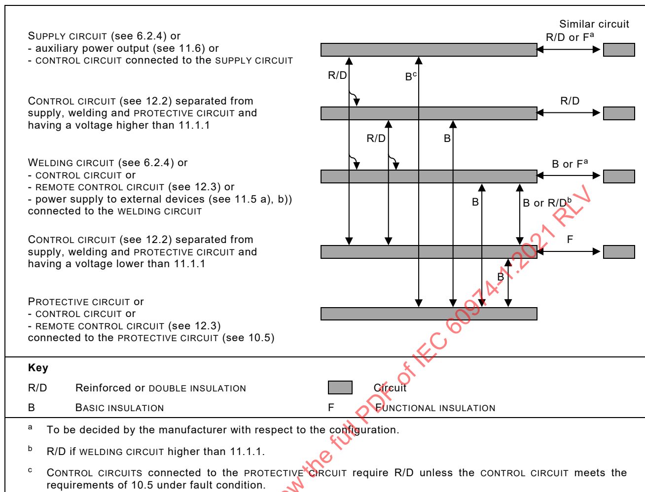
Figure 2 – Example of insulation configuration for CLASS I EQUIPMENT
